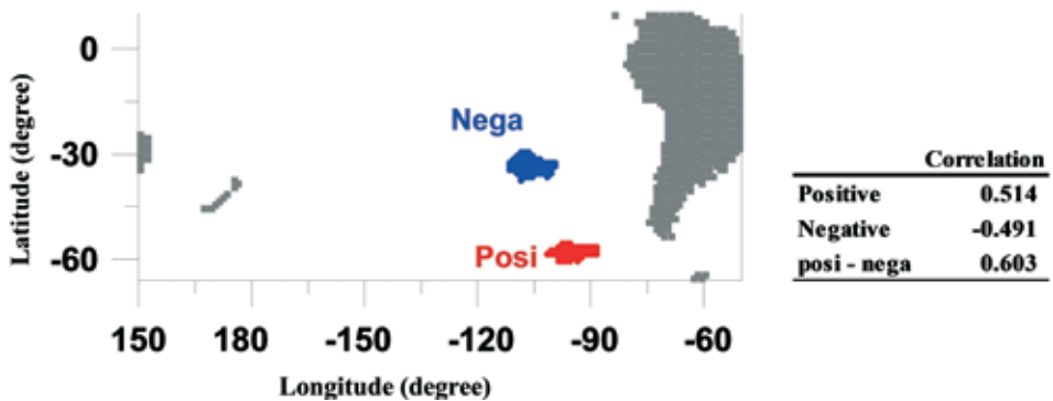
Figure 5-2. Vegetation zone ST summer rainfall significant SST dipole areas ( |r| > 0.43 , lag 5 months).
