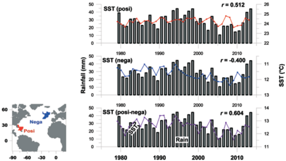
Figure 5-1. Vegetation zone DS summer rainfall significant SST dipole areas. Right: SST dipole difference and corresponding summer rainfall ( |r| > 0.33 , lag 5 months).
