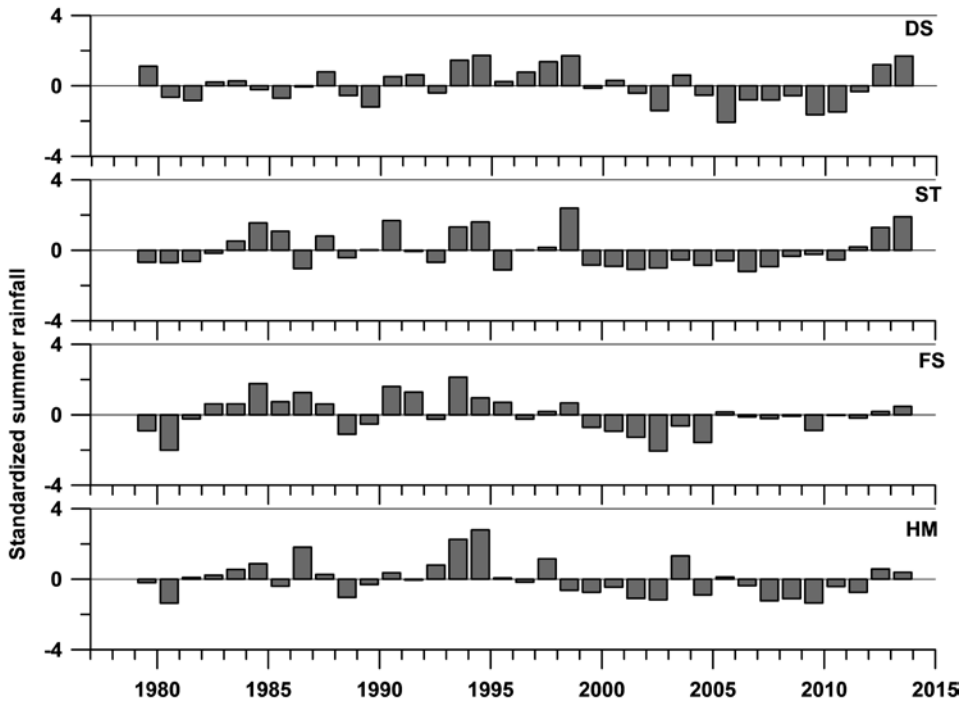
Figure 3. Standardized summer rainfall (3 months; JJA) in the four investigated vegetation zones.
