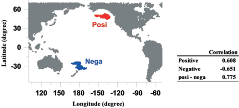
Figure 5-4. Vegetation zone HM summer rainfall significant SST dipole areas ( |r| > 0.53 , lag 5).
