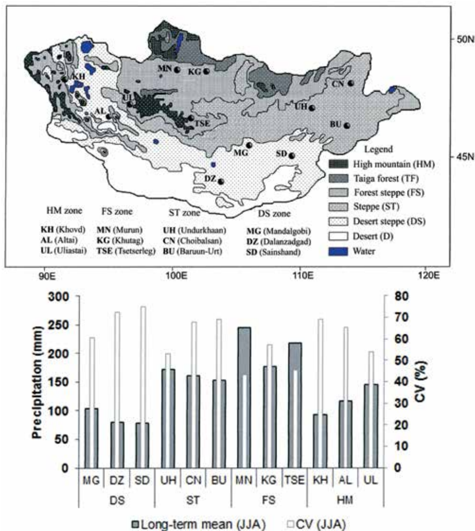
Figure 1. Vegetation zones in Mongolia. Summer rainfall for the four major vegetation zones, namely desert steppe (DS), steppe (ST), forest steppe (FS), and high mountain (HM), was investigated in this paper ( above ). Mean precipitation and CV of stations ( below ).
